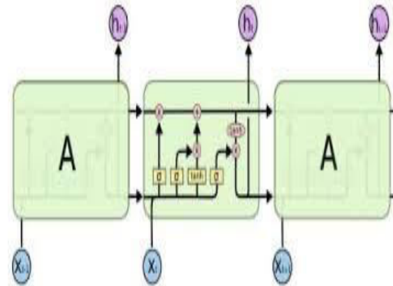
Figure 2. An LSTM Architecture [15]
