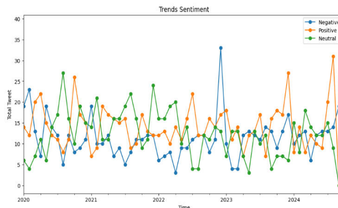
Figure 5. Trend Sentiment
