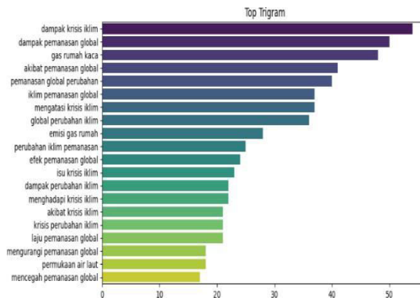
Figure 4. Top Trigram
