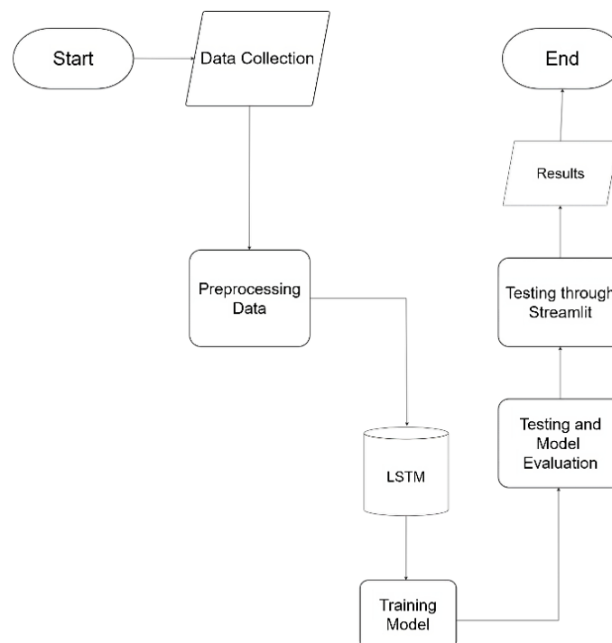
Figure 1. Research Flowchart
