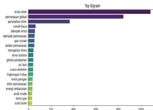
Figure 3. Top Bigram
